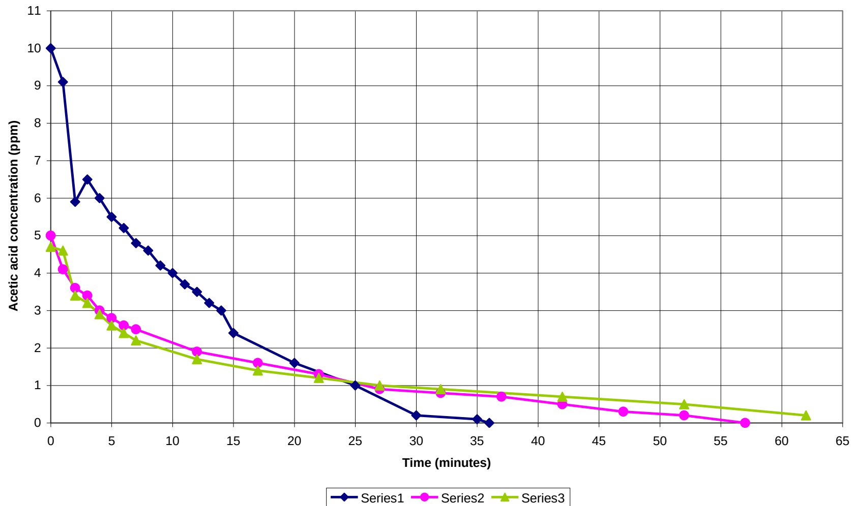
Figure A-2: 2006 Acetic Acid Absorption Test Results
